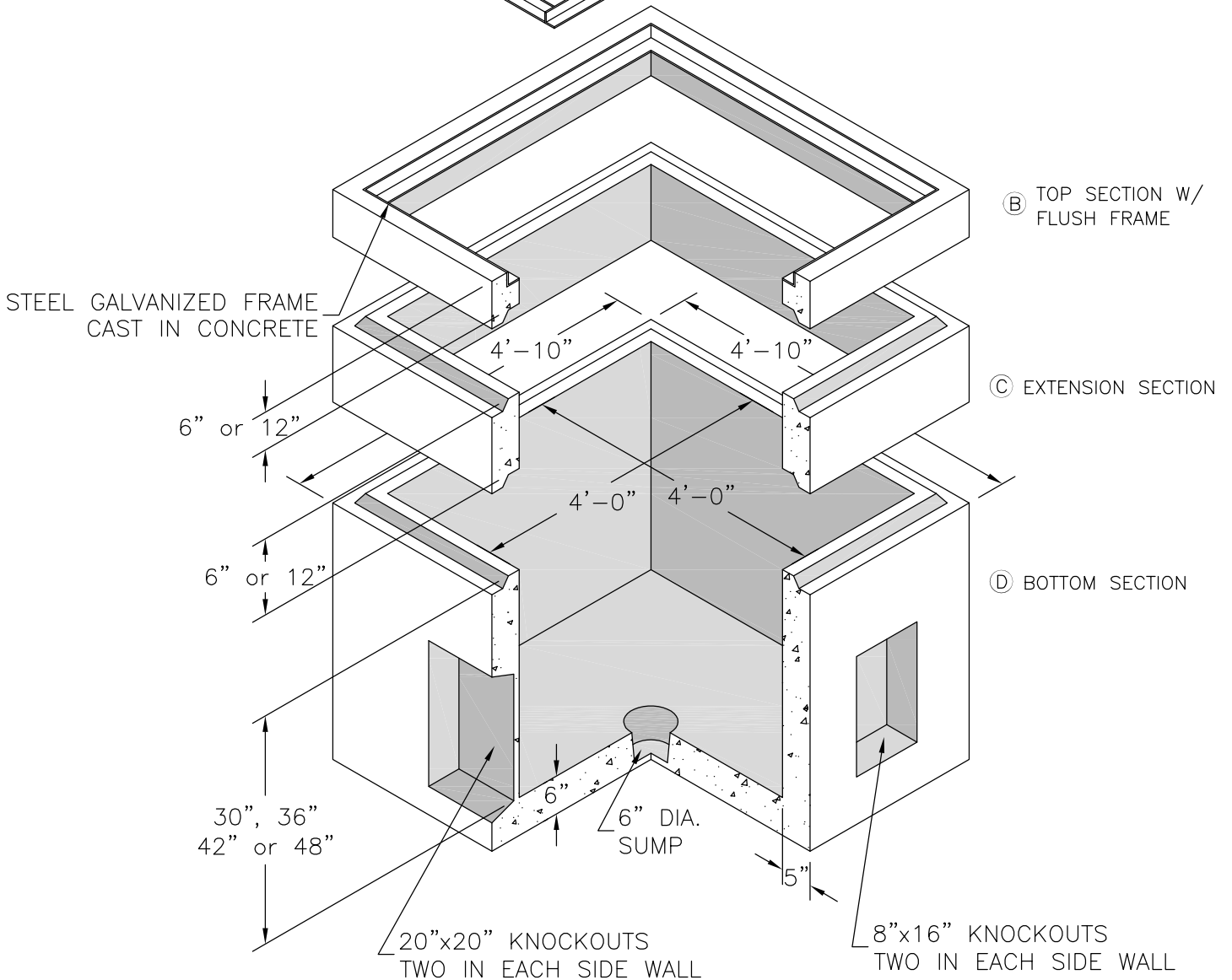
(A) 2pc. STEEL BOLTDOWN TRAFFIC / PARKWAY COVER
