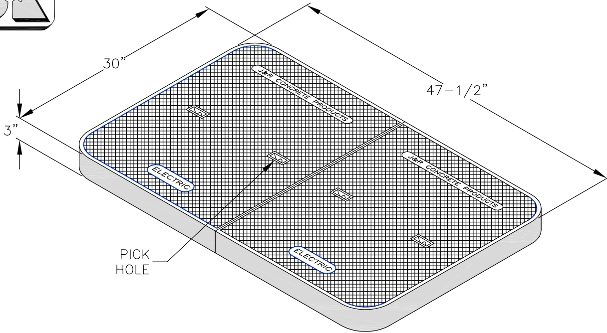
POLYMER CONCRETE COVER (2 HALVES)
