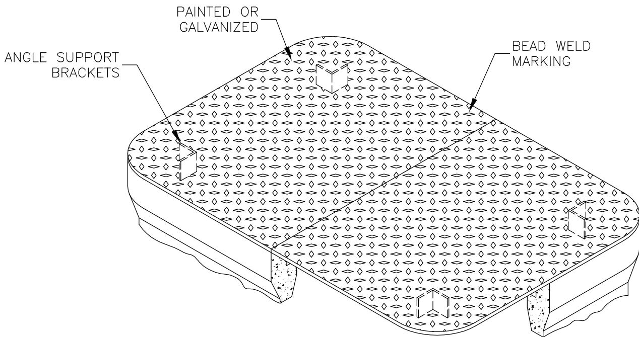
STEEL SUPERIMPOSED COVER (2 HALVES)
