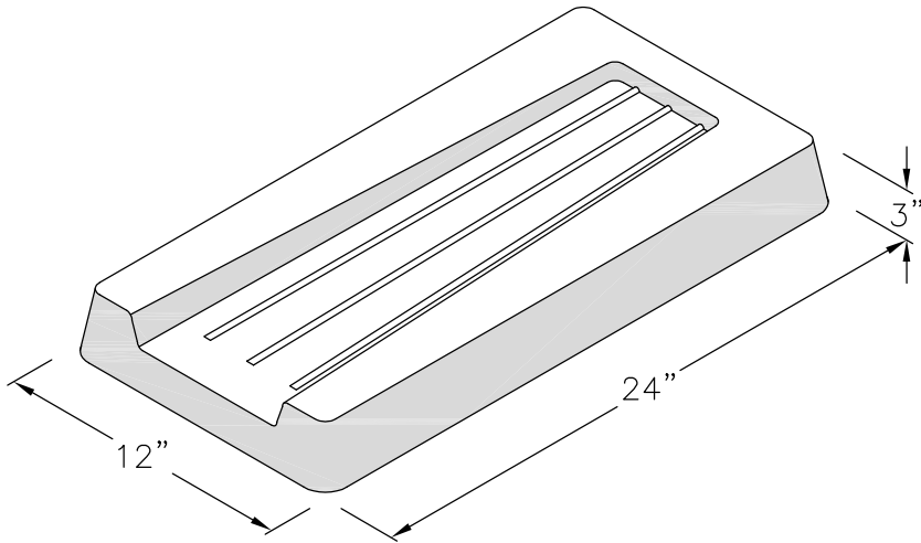
1-SBP 12"X24" SPLASH BLOCK
