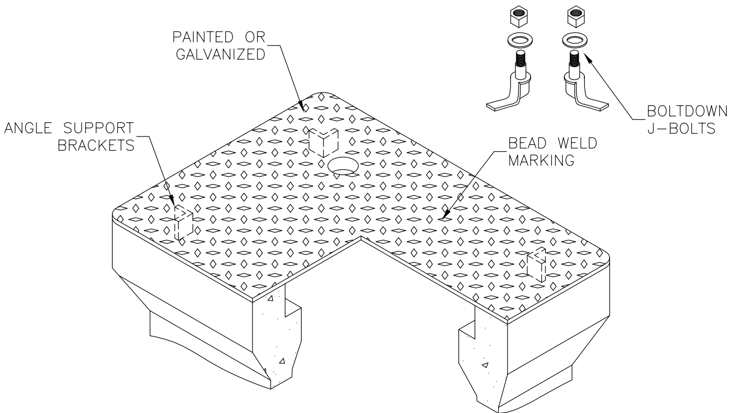
STEEL BOLTDOWN SUPERIMPOSED COVER
