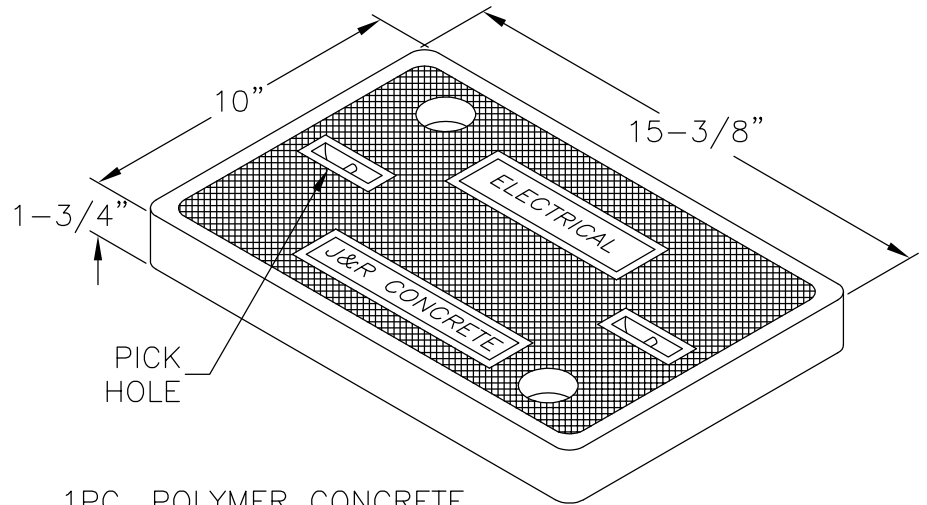
1PC. POLYMER CONCRETE BOLTDOWN COVER
